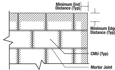
Wall Face Permissible Anchor Locations (Un-hatched Area)
