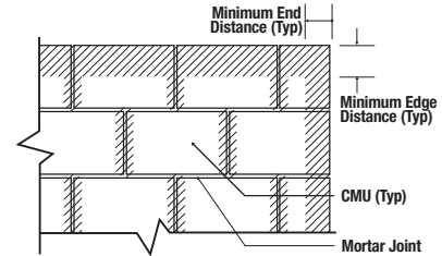
Wall Face Permissible Anchor Locations (Un-hatched Area)
